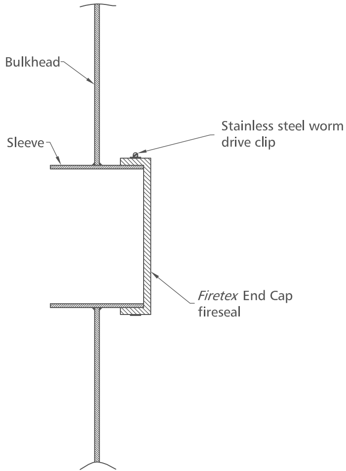
(SECTIONAL VIEW)
